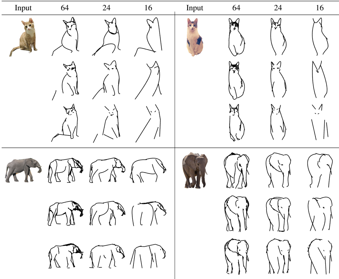
Figure 47. Sketches produced by our method with different styles and levels of abstraction. The columns indicate the total number of control points used to generate the sketch - 64, 24, and 16. The rows indicate the number of control points used for each stroke, which defines the style - 4, 3, and 2 control points respectively.
