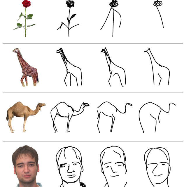
Figure 3. Different levels of abstraction produced by our method. Left to right: input images and increased level of abstraction, achieved by reducing the number of strokes used by half each column.
