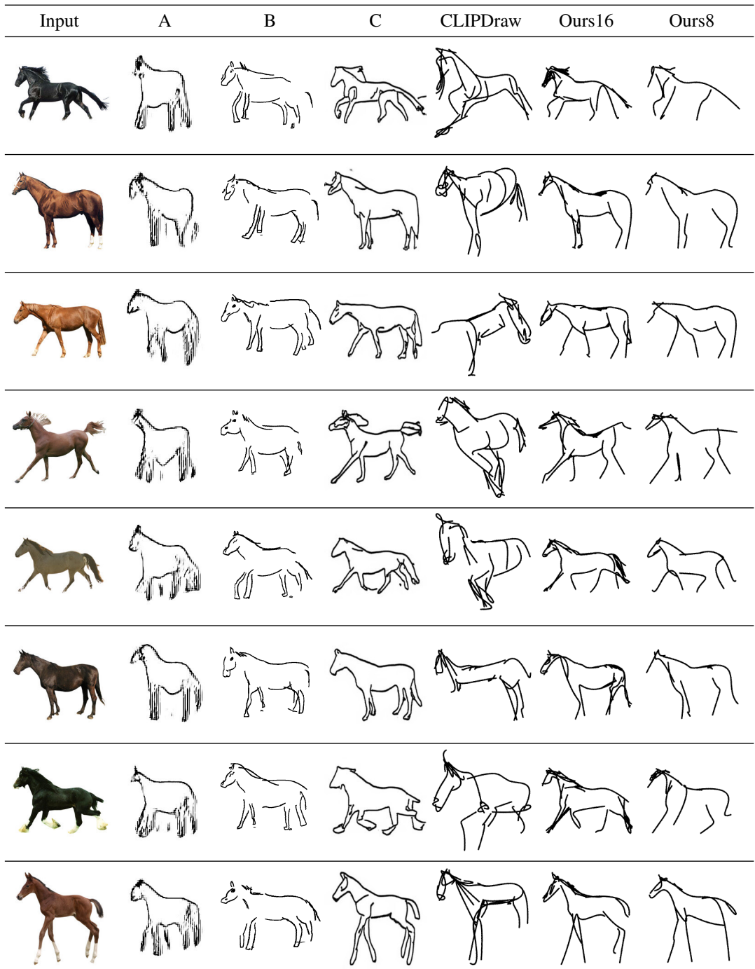
Figure 42. Comparison to competitor methods on images from the "horse" class. Left to right : (A) Kampelmühler and Pinz [21], (B) Li et al. [25], (C) Li et al. [23], and CLIPDraw [11].
