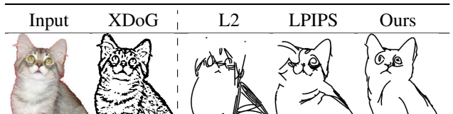
Figure 6. Loss functions comparison — we optimize the strokes by minimizing different losses: L2 loss simply encourages the filling of colored pixels, LPIPS is more semantically aware, but the resulting sketch is still close to the edge map (see the XDog edges for comparison). In contrast, our CLIP-based loss allows better semantic depiction while preserving the morphology of the subject.
